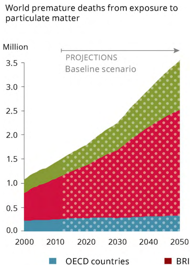
Premature deaths due to particulate matter and ground-level ozone, 2000–2050
