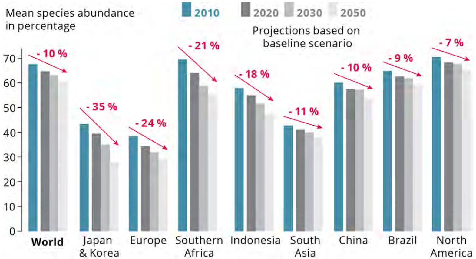
Terrestrial mean species abundance, 2010–2050
